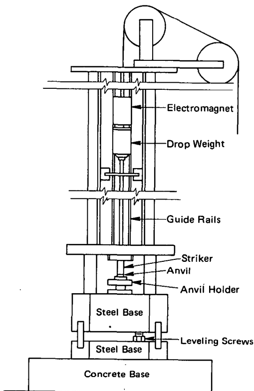
Fig 2. Drop Weight Impact Machine, ERL Model, type 12 tools
